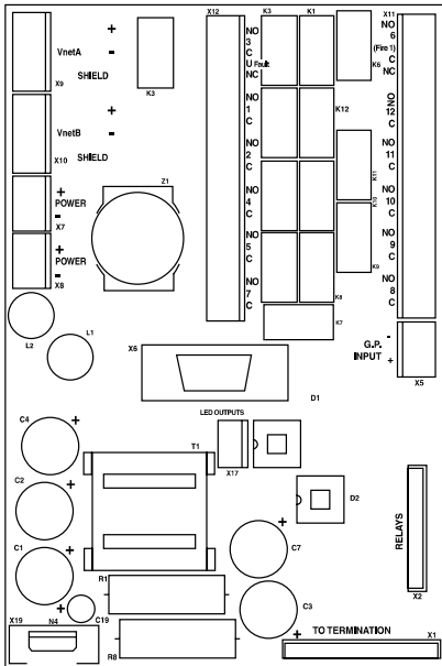
Detector Termination Card 12 Relay Version
