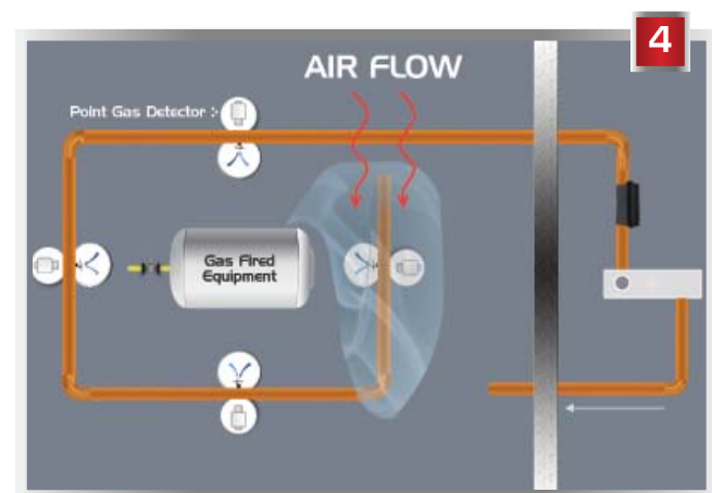
Figures 3 + 4 – Demonstrate the design flexibility of VESDA ECO. Knowing where a leak will occur is always a judgement call. In this example, four conventional point gas detectors are required to cover the same area as one VESDA ECO detector. VESDA ECO provides a more cost-effective solution.
